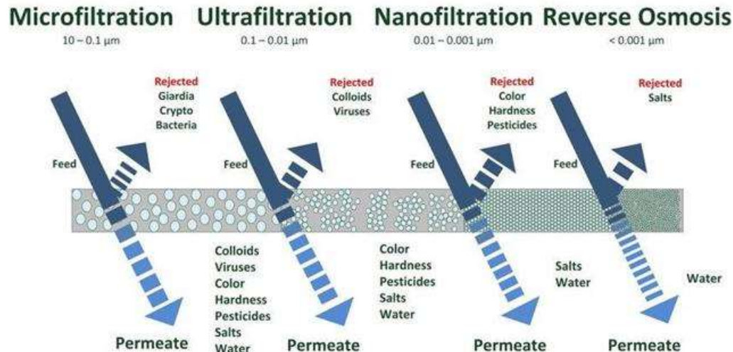
Fig. 7 Classification of pressure driven membranes and schematic illustrations of their operation are according to the pore size.
