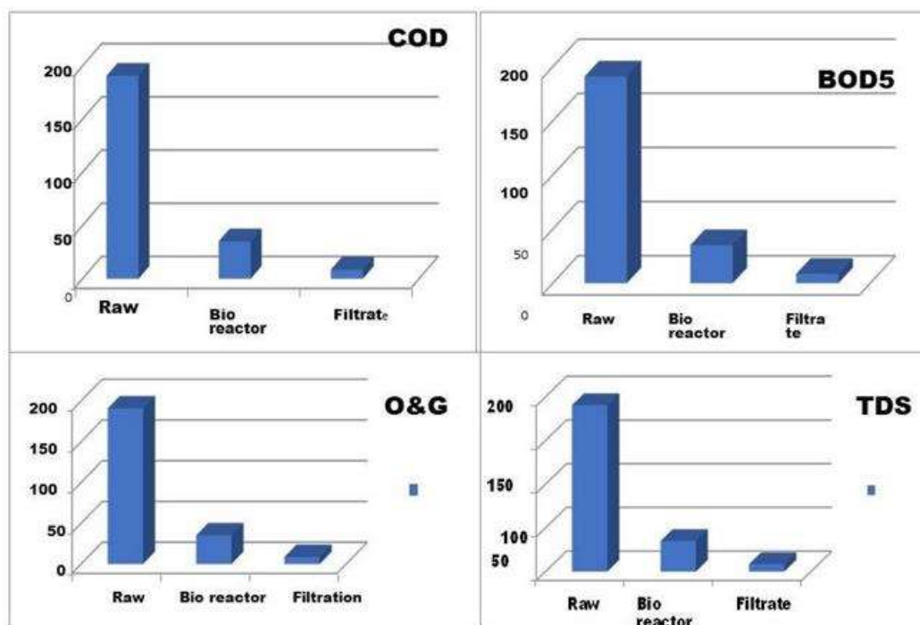
Fig. 11 Graphs shows physicochemical parameters of raw water, after bio-reactor treatment and permeates water after UF filtration
