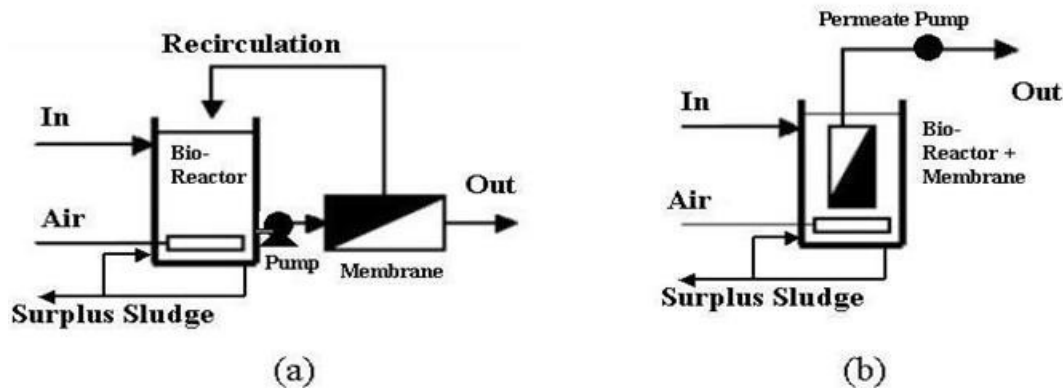
Fig. 6 (a) Side stream MBR (b) Submerge MBR
