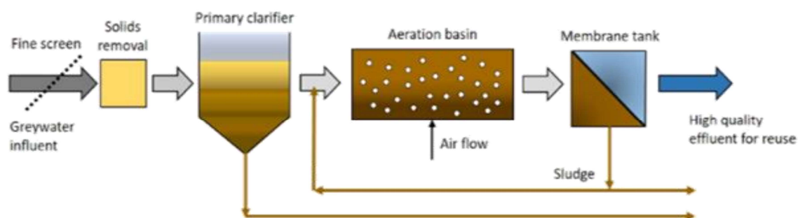
Fig. 8 Schematic diagram of Greywater treatment with MBR Bio-reactor (MBR) technology [4].
